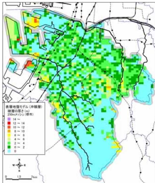
(c) 礫層
