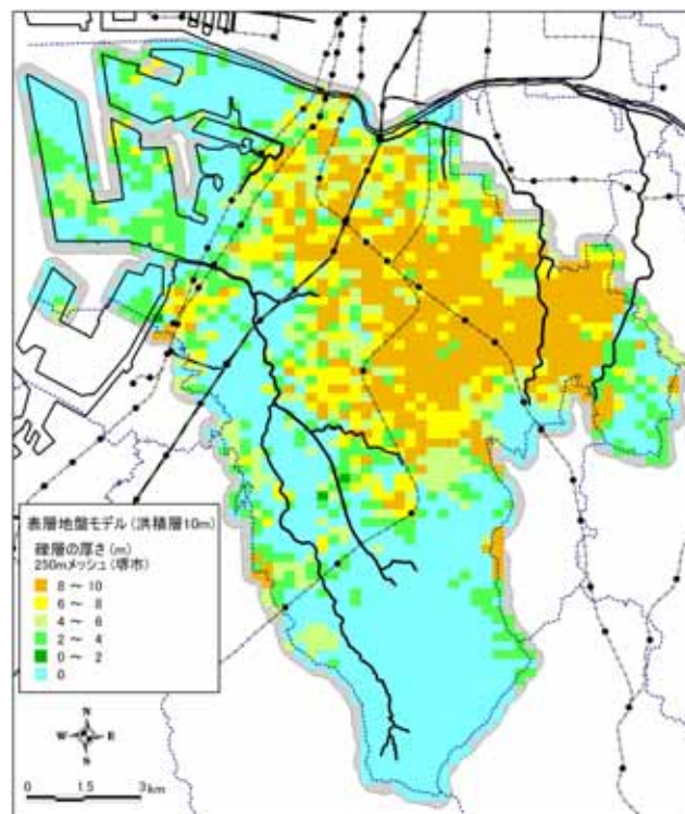
(c) 礫層
